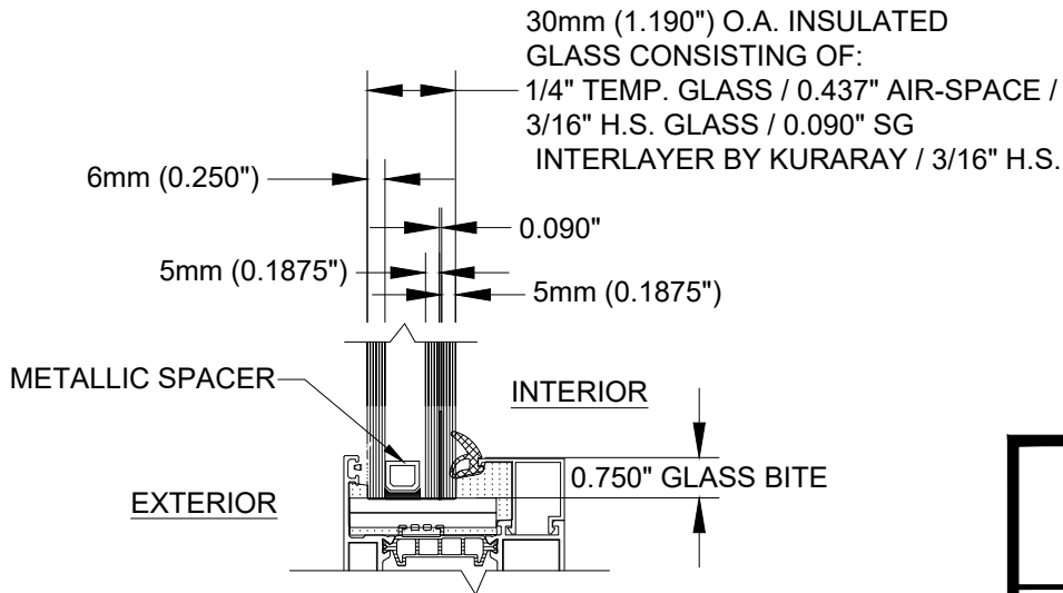
GLAZING DETAIL 1
