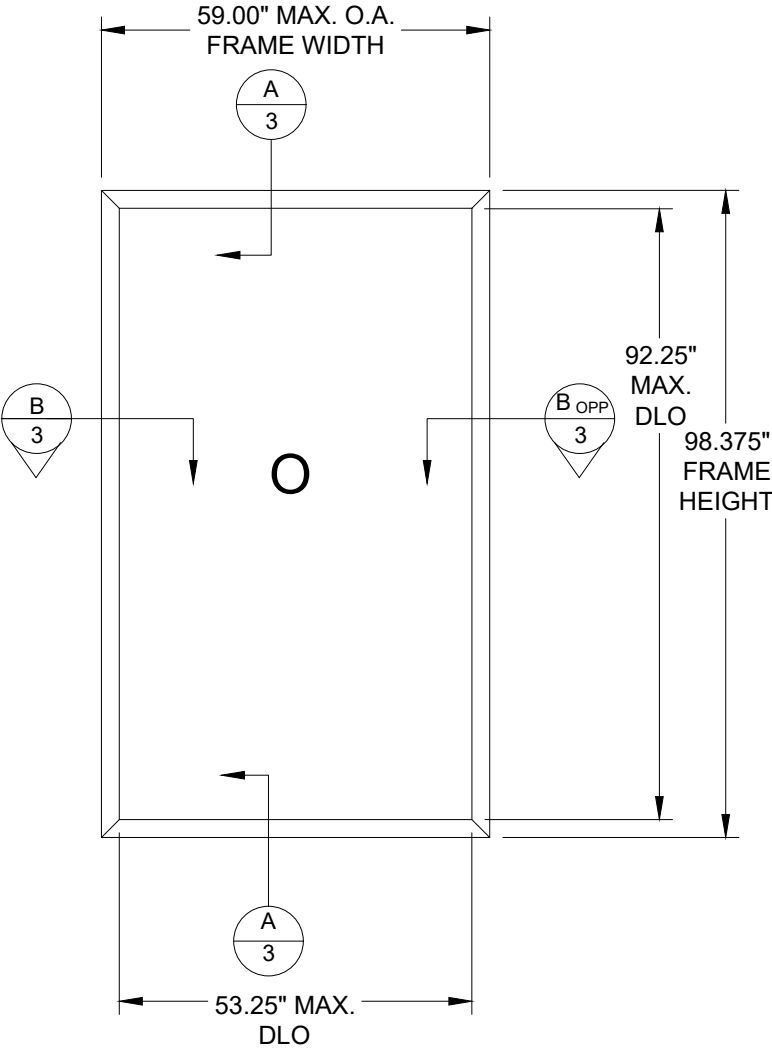
ELEVATION LAYOUT PICTURE WINDOW
