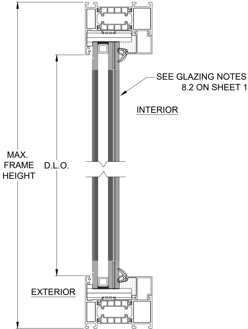
A 3 VERTICAL SECTION
