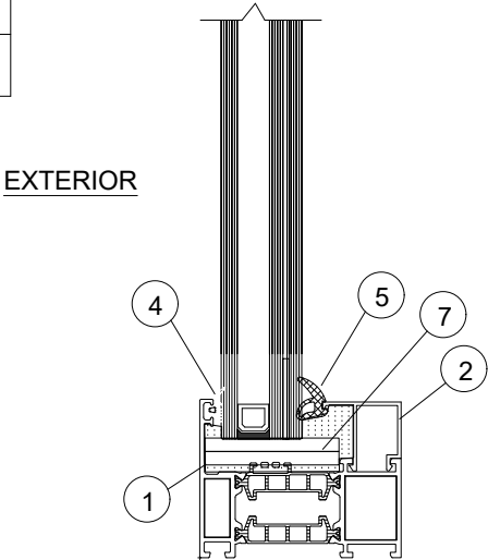
TYPICAL CROSS SECTION FOR PARTS IDENTIFICATION EQUAL LEG FRAME
