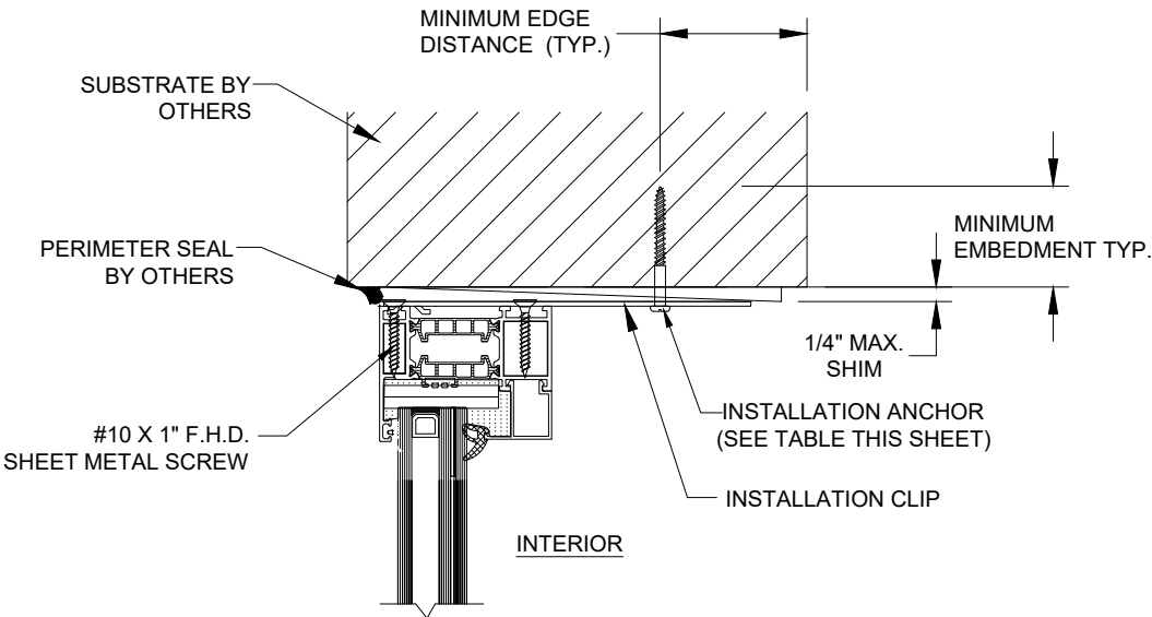
B 4 ANCHOR DETAIL INSTALLATION CLIP FRAME HEAD
